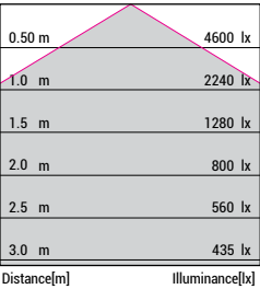
NRI 90 LED PS 10920 lm 4000k 96w
